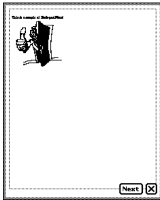
Print Preview
